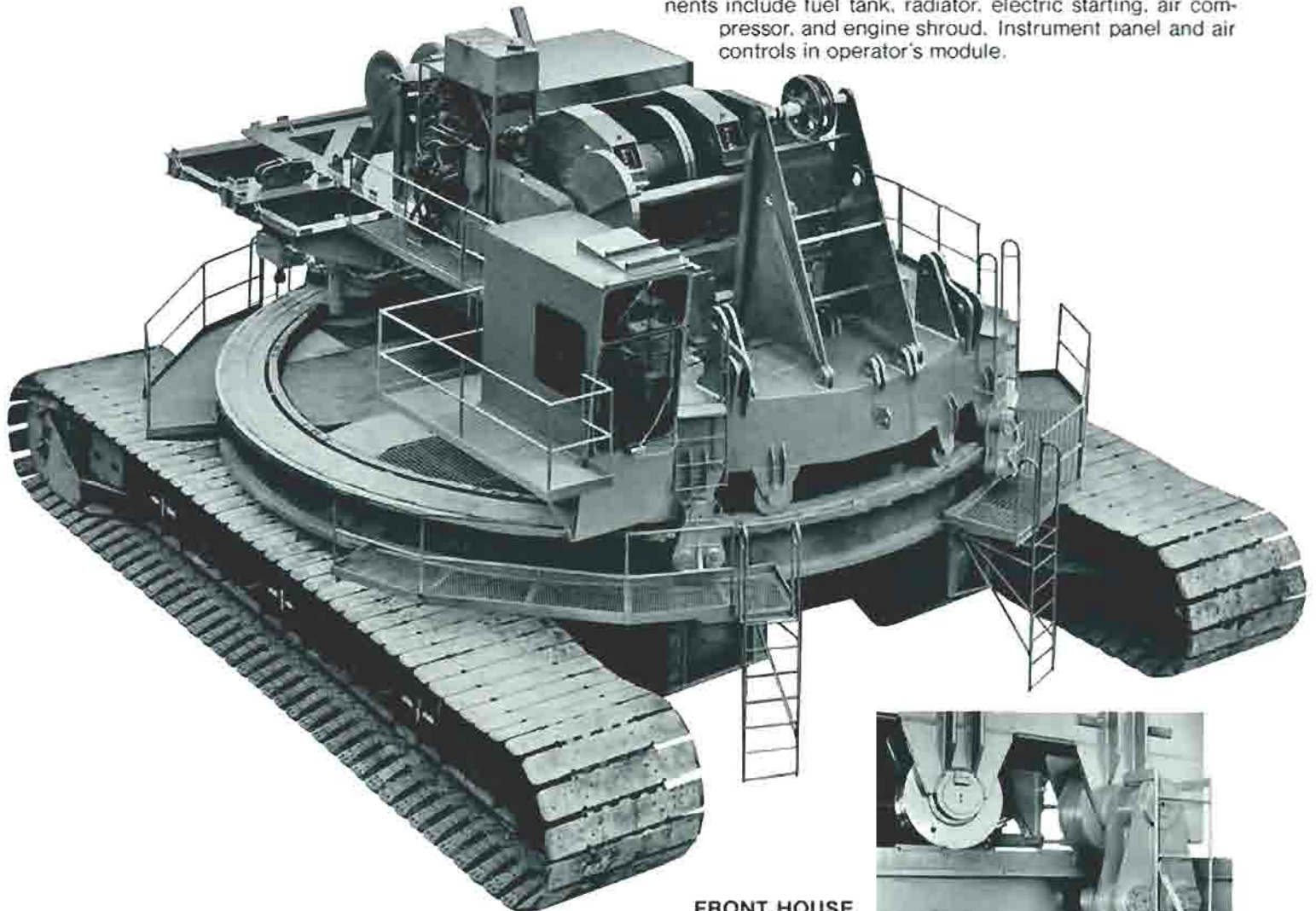
FRONT HOUSE AND HOOK ROLLERS
